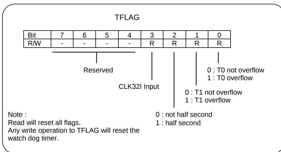
Figure 17. Timer Flag Status Register/Watch-dog Reset
