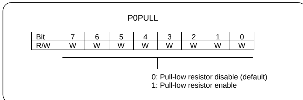
Figure 12. Port 0 Pull-low Control Register
