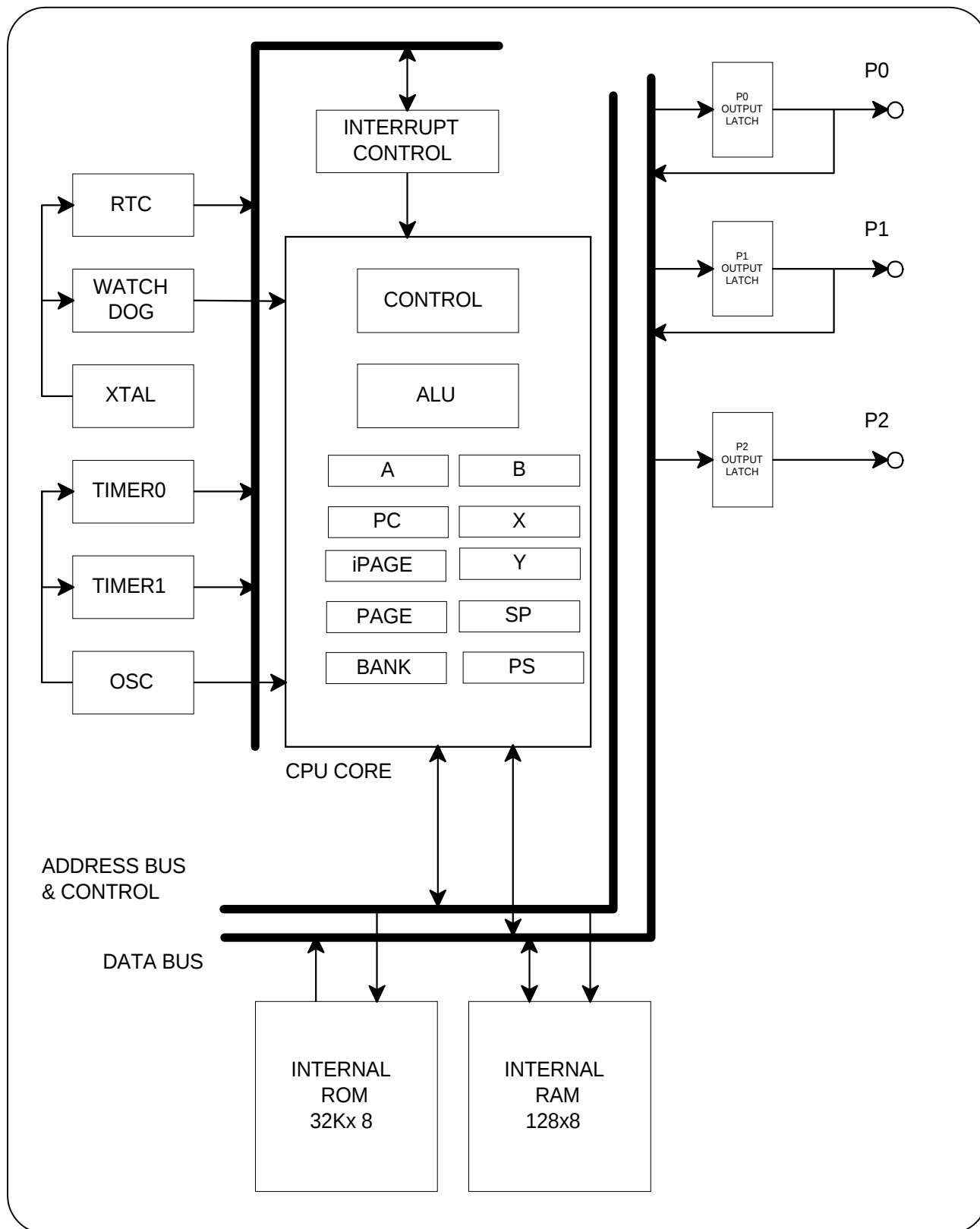
Figure 4. Block diagram of SCG9832
