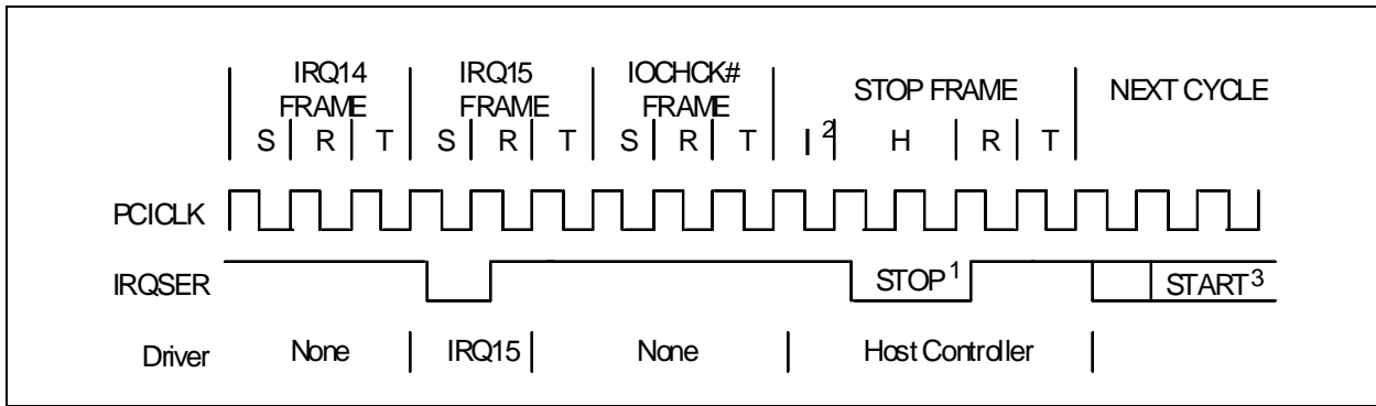
FIGURE 8-3: SERIAL INTERRUPT WAVEFORM “STOP FRAME”
