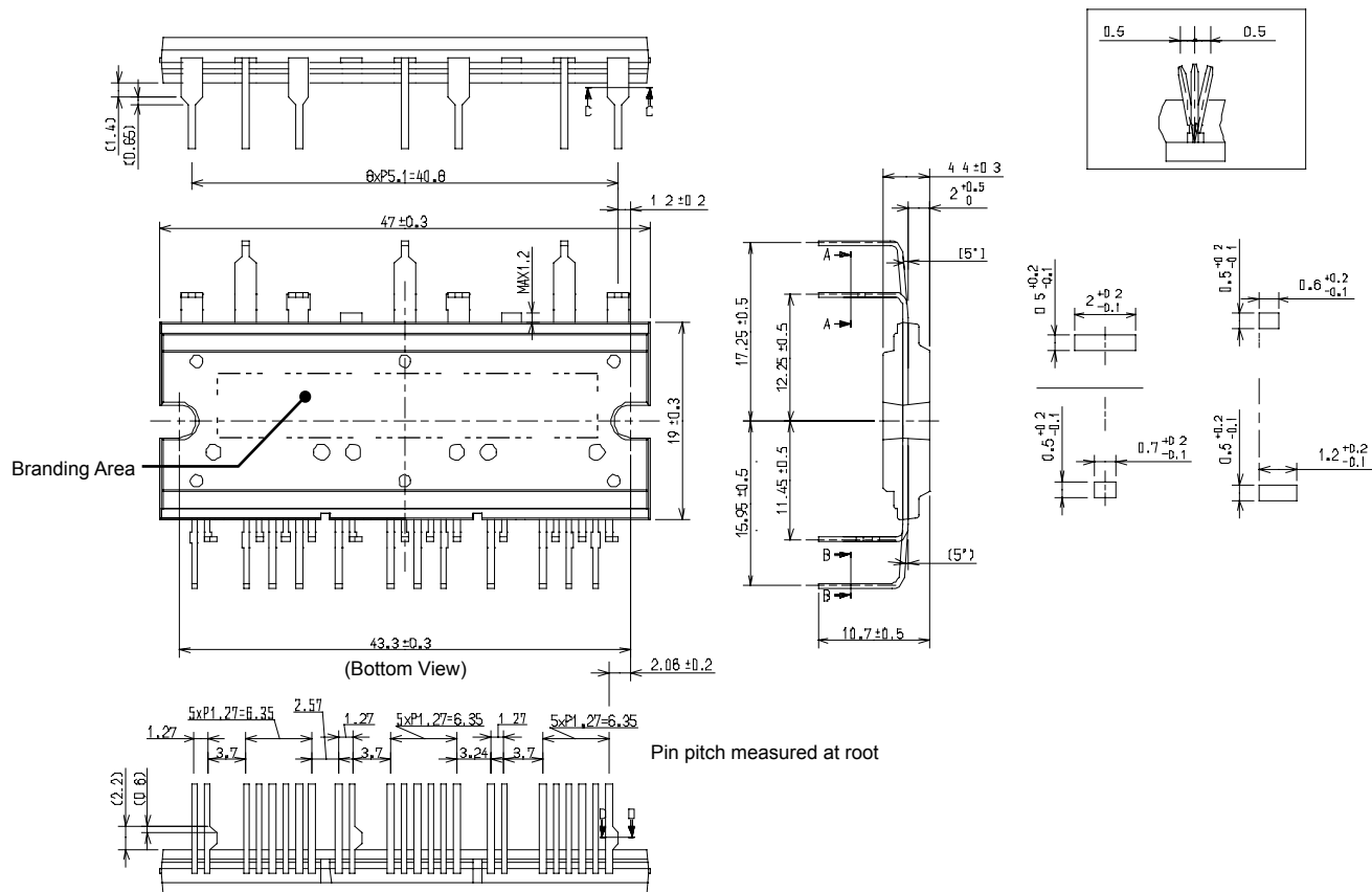
PACKAGE OUTLINE DRAWING
