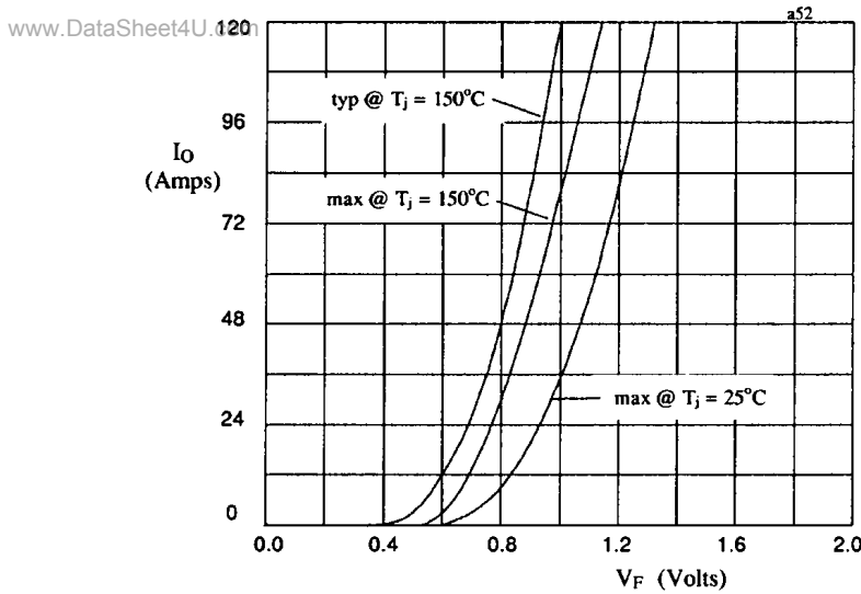
Fig 1. Forward voltage drop against current (per leg)
