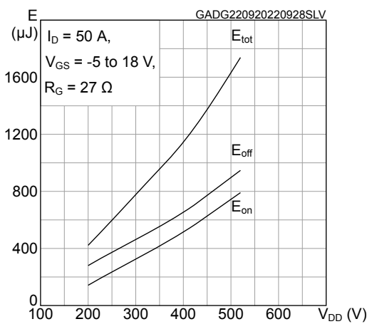
Figure 10. Typical switching energy vs V_DD
