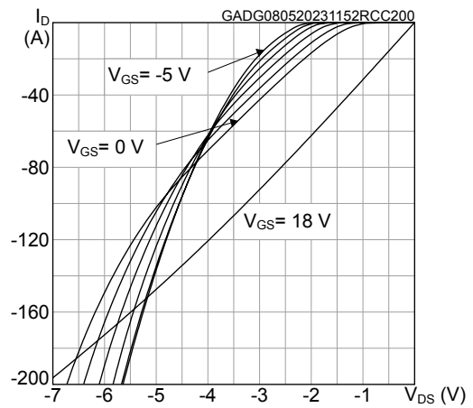
Figure 16. Typical reverse conduction characteristics ( T_J = 200 \text{ }^\circ\text{C} )
