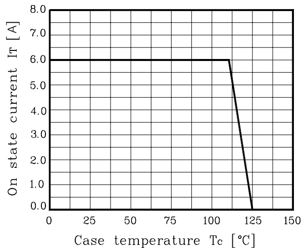
Fig. 2 I_{T(RMS)} - T_c
