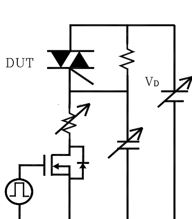
Simple circuit for (dV/dt)_S
