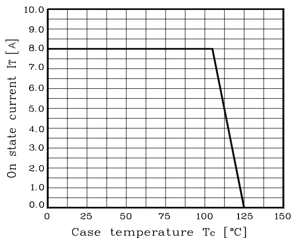
Fig. 2 I_{T(RMS)} - T_C
