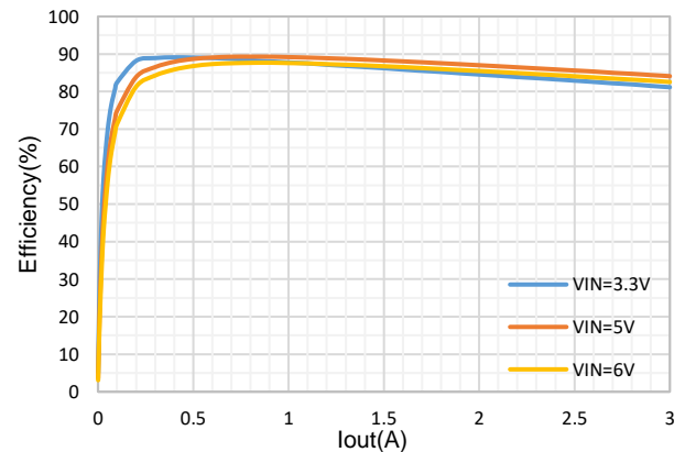
Efficiency, Vout=1.2V
