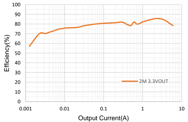
Figure 5. Efficiency, F_{SW}=2MHz , V_{in}=12V , V_{OUT}=3.3V
