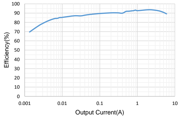
Figure 3. Efficiency, F_{SW}=400KHz , V_{OUT}=3.3V
