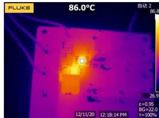
Figure 23. Thermal, 24VIN, 3.3Vout, 3A
