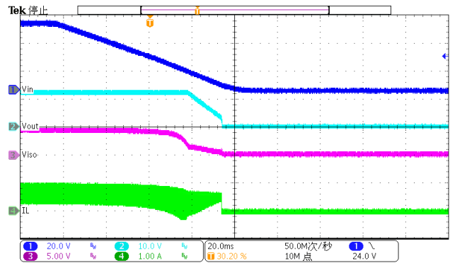
Figure 26. Power down(Io=0.6A, liso=0.5A)
