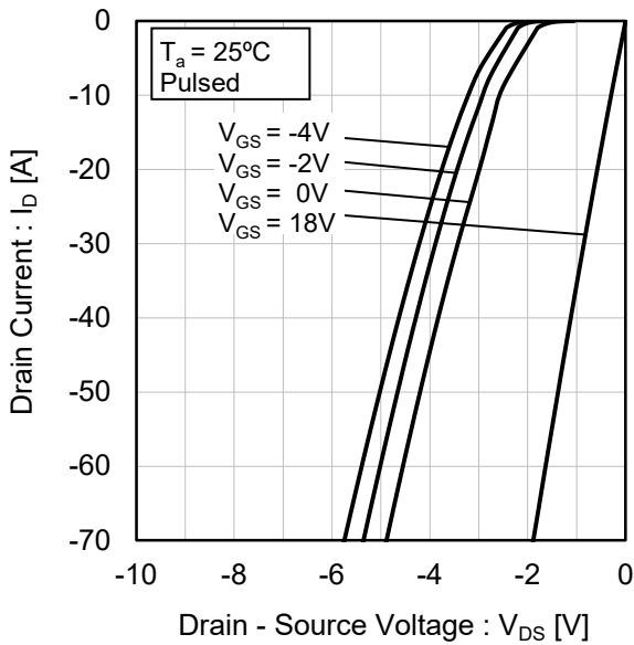
Fig.6 T_j = 25^\circ C 3rd Quadrant Characteristics
