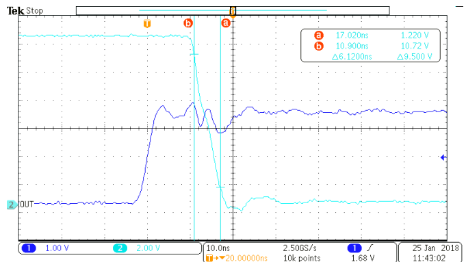
Figure 15. IN- Switching OFF
