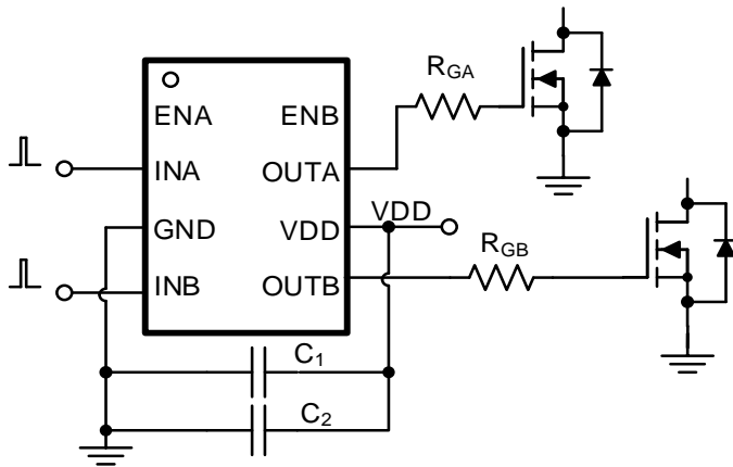
SCT52240 Typical Application
