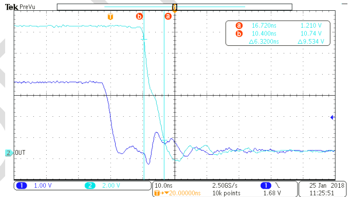
Figure 13. IN+ Switching OFF
