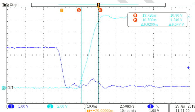
Figure 14. IN- Switching ON
