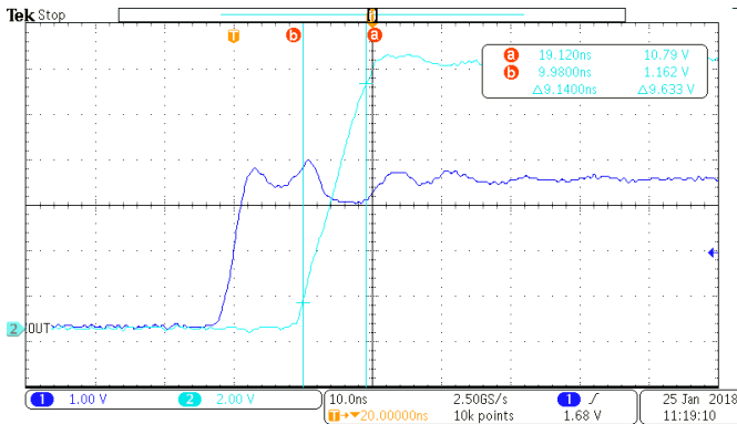
Figure 12. IN+ Switching ON
