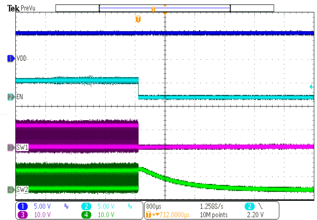
Figure 15. EN Shutdown
