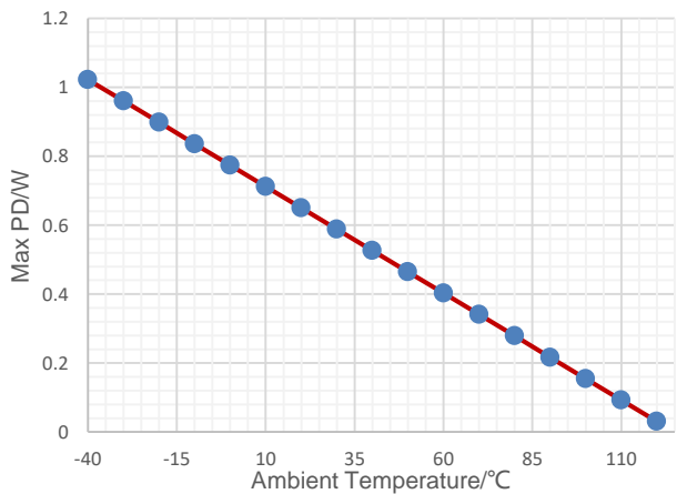
Figure 27. Maximum Allowed Power Dissipation vs Ambient Temperature, SOT23-5, T_J \leq 125^\circ\text{C}
