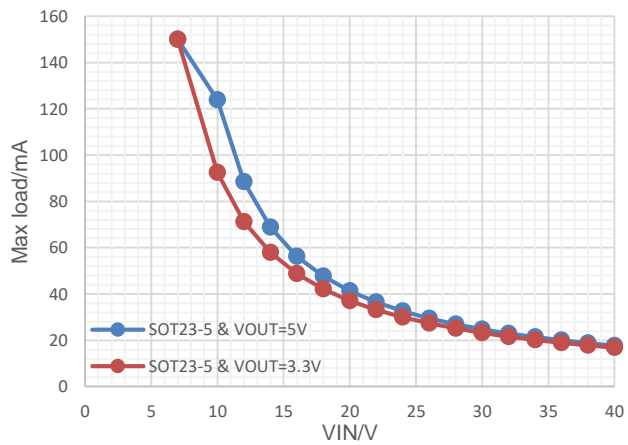
Figure 28. Maximum Output Current vs Input Voltage, SOT23-5, T_J \leq 125^\circ\text{C}
