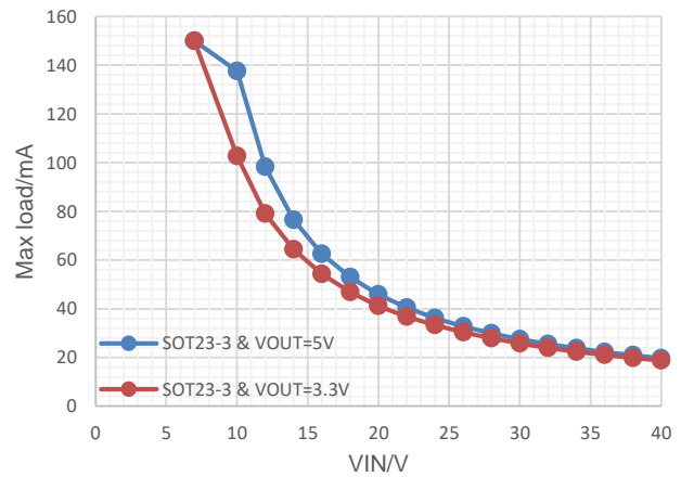
Figure 26. Maximum Output Current vs Input Voltage, SOT23-3, T_J \leq 125^\circ\text{C}
