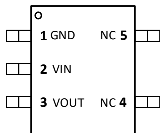
SCT71401Fxx-TWDR SOT23-5 Package
