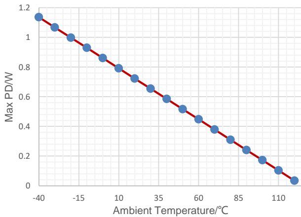
Figure 25. Maximum Allowed Power Dissipation vs Ambient Temperature, SOT23-3, T_J \leq 125^\circ\text{C}
