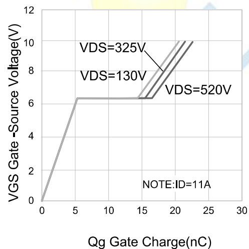
Figure 6. Charge Quantity Characteristics
