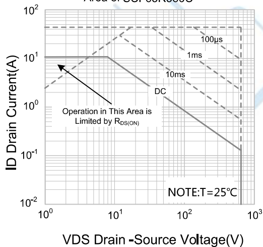
Figure 9-3. Max. Safe Operating Area of SCP65R380C
