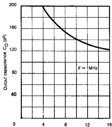
OUTPUT CAPACITANCE vs COLLECTOR BASE VOLTAGE
