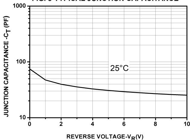
FIG. 5-TYPICAL JUNCTION CAPACITANCE
