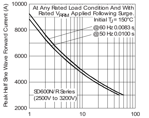
Fig. 11 - Maximum Non-Repetitive Surge Current
