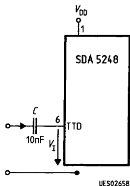
Test Circuit 2
