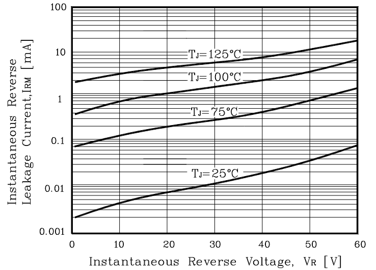
Fig. 2) Typical Reverse Characteristics (Per diode)
