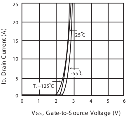
Figure 2. Transfer C Characteristics
