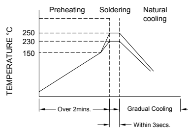
Figure 2. Wave Soldering
