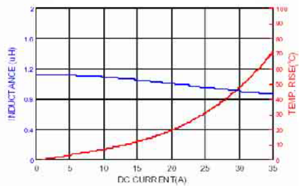
SDL1108-1R2MF
