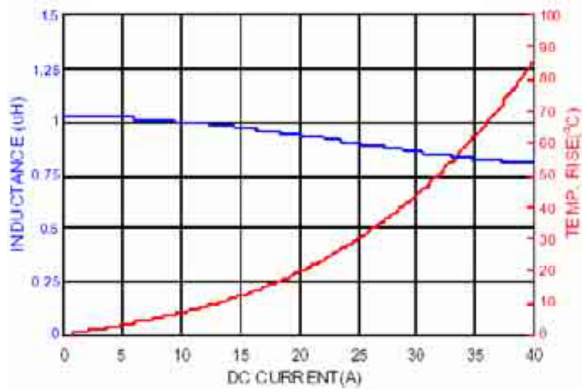
SDL1108-1R0MF
