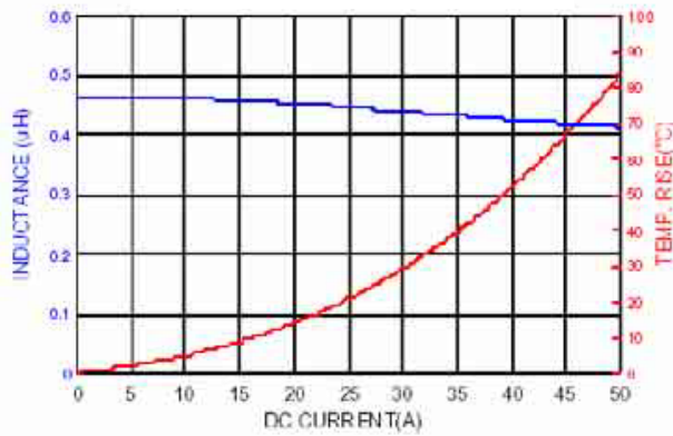
SDL1108-R47MF
