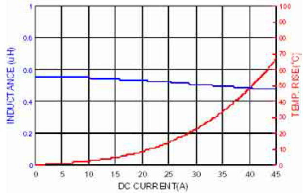
SDL1108-R60MF
