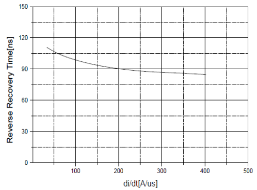
Figure 2. Typical Reverse Recovery Time vs. -di/dt
