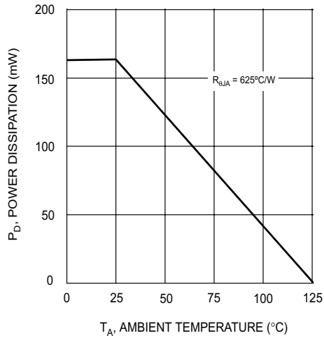
Fig. 1 Derating Curve
