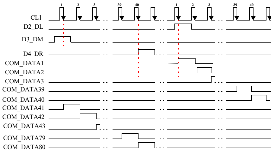
Fig.27 SHL=LOW, dual-type interface mode.
