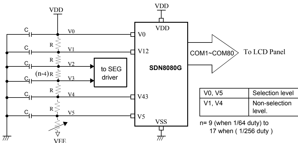
Fig.6 COMMON driver application.
