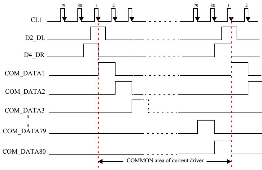
Fig.25 SHL=LOW, single-type interface mode.
