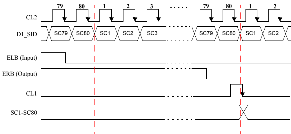
Fig.24 SHL=HIGH, 1-bit serial mode interface.
