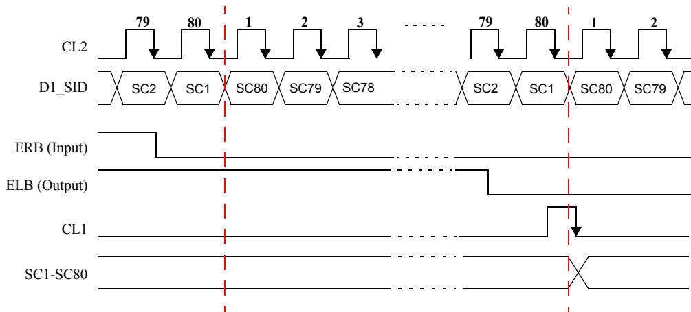
Fig.23 SHL=LOW, 1-bit serial mode interface.
