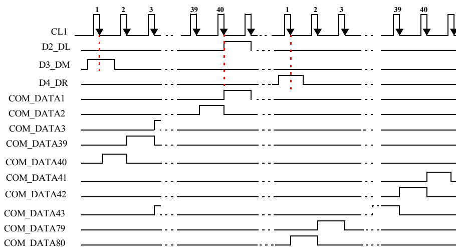
Fig.28 SHL=HIGH, dual-type interface mode.
