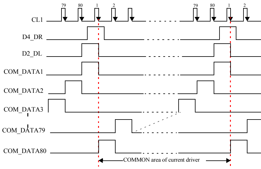
Fig.26 SHL=HIGH, single-type interface mode.
