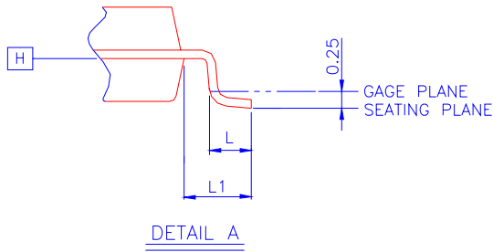
SDN8080G LQFP100 Package Outline Drawing
