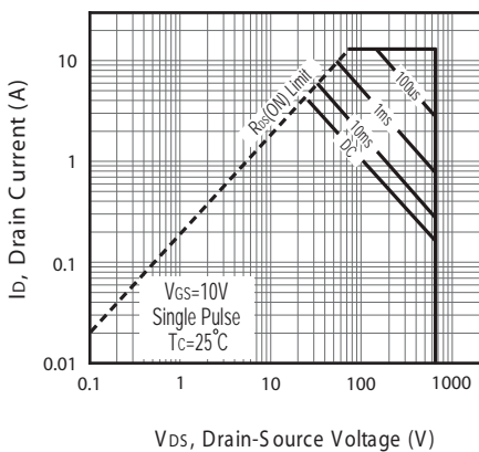
Figure 11a. Maximum Safe Operating Area for SDP04N65
