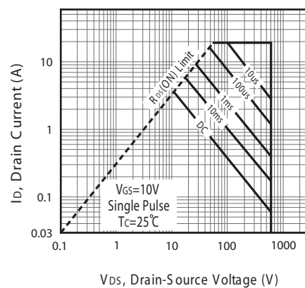
Figure 11b. Maximum Safe Operating Area for SDF06N60
