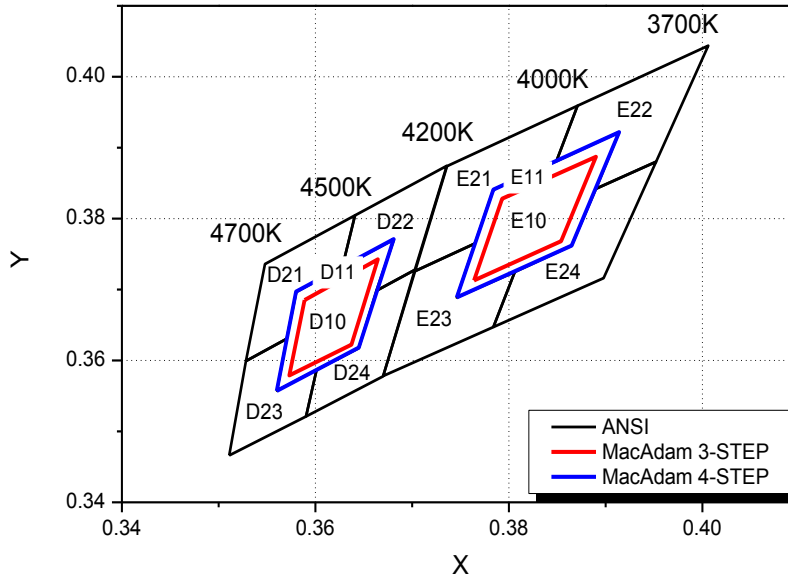
CIE Chromaticity Diagram, T_j=25^\circ\text{C} , I_f=700\text{mA}
