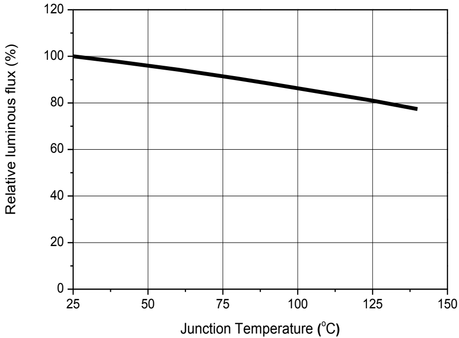
Fig 7. Junction Temperature vs. Relative Light Output, I_F=700\text{mA}
