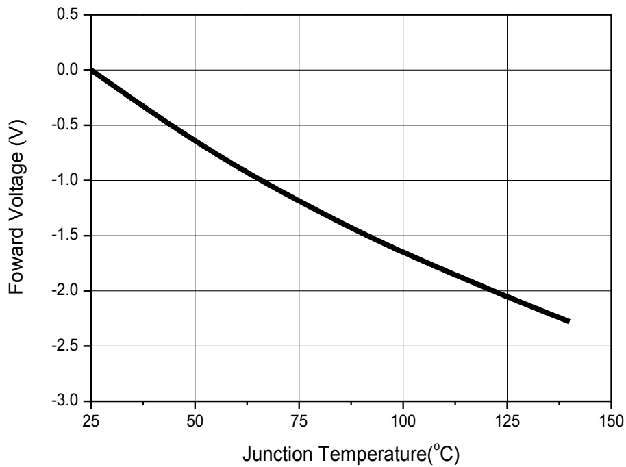
Fig 8. Junction Temperature vs. Forward Voltage, I_F=700\text{mA}
