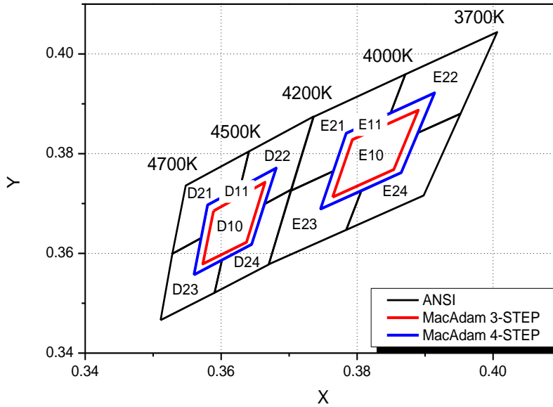
CIE Chromaticity Diagram, T_j=25^\circ\text{C} , I_F=1.5\text{A}
