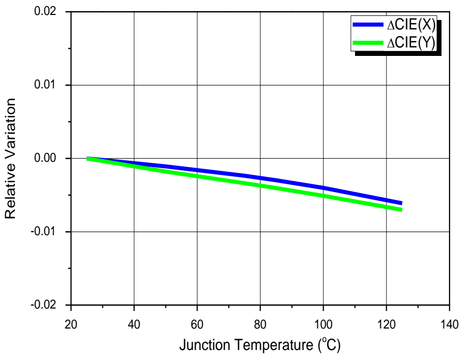
Fig \6. Junction Temperature vs. CIE X, Y Shift, I_F=1.5A (Warm white)
