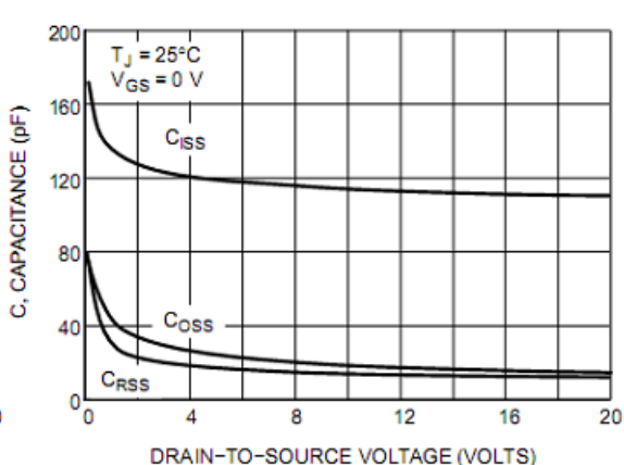
Figure 6. Capacitance Variation
