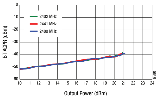
Figure 14. BT ACPR CH+3 vs P out , BT-BDR-DH1
