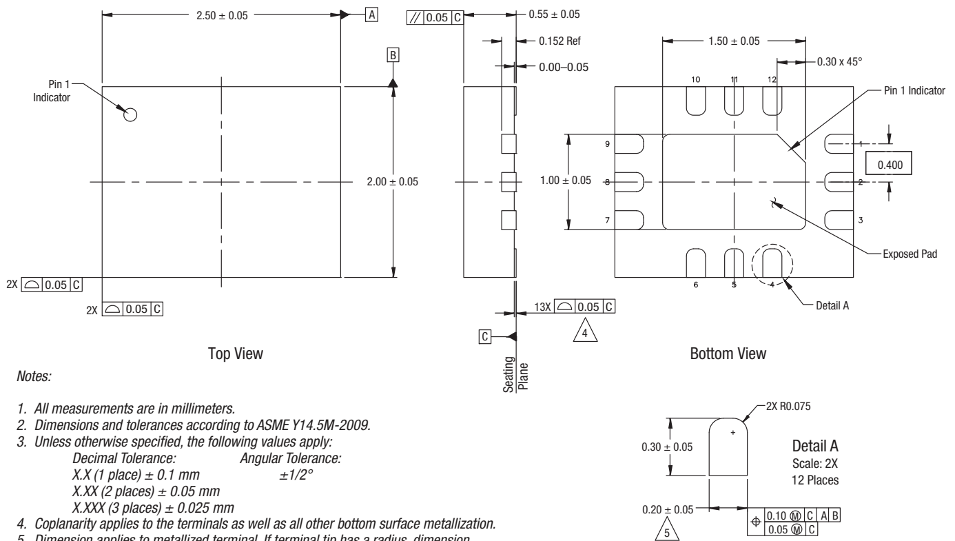
Figure 20. SE2433T Package Dimensions
