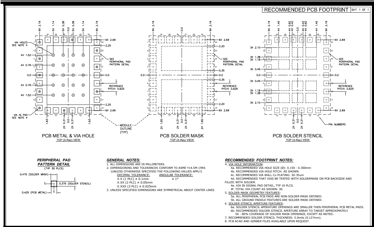
Figure 5: Recommended Land and Solder Patterns
