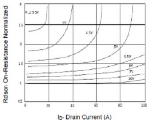
Figure 3 Rds(on)-Drain Current
