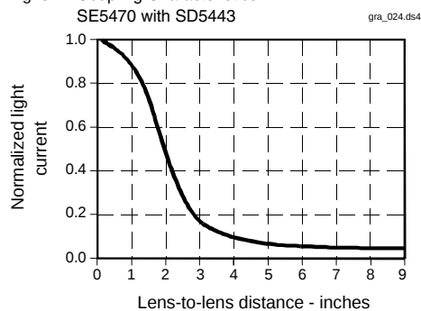
Fig. 9 Coupling Characteristics SE5470 with SD5443
