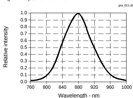
Fig. 7 Spectral Bandwidth
