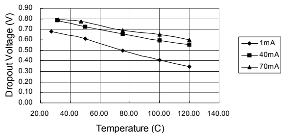
Dropout Voltage vs Temperature
