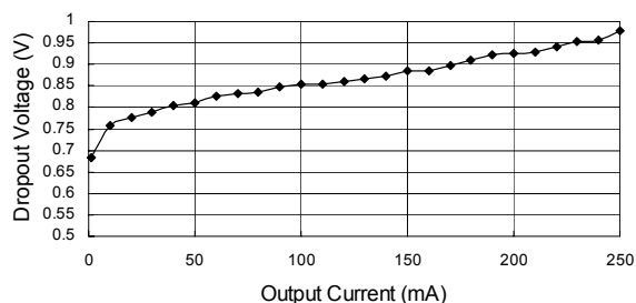
Dropout Voltage vs Output Current
