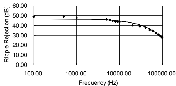
Ripple Rejection
