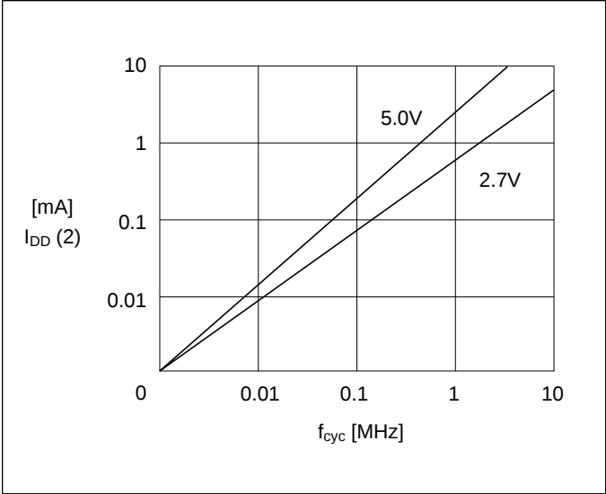
Figure 3.4 Power consumption during CPU access cycle (I DD [2])
