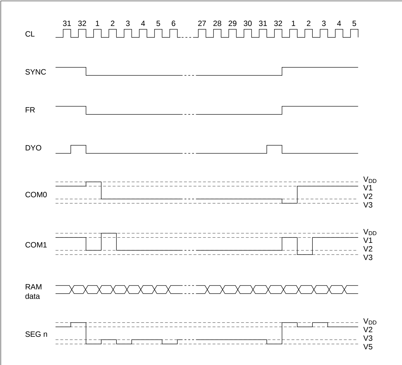
Figure 4.7 Frame driver timing for duty 1/32
