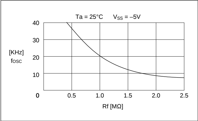
Figure 3.1 Oscillator frequency vs. frame vs. f_F [SED1560 Series]
