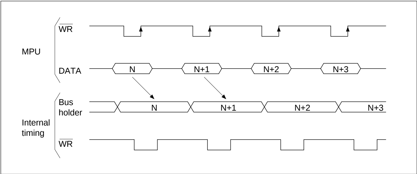
Figure 4.2 Write timing
