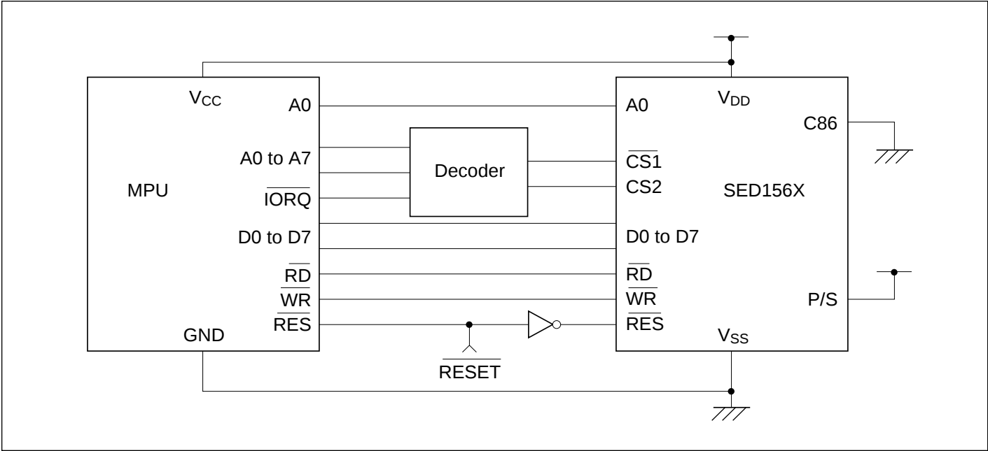
Figure 5.6 8080-series microprocessors
