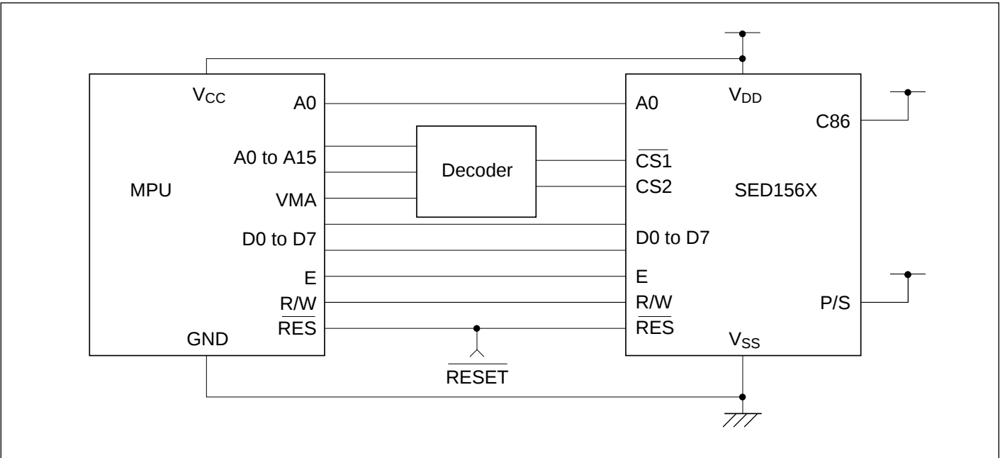
Figure 5.7 6800-series microprocessors
