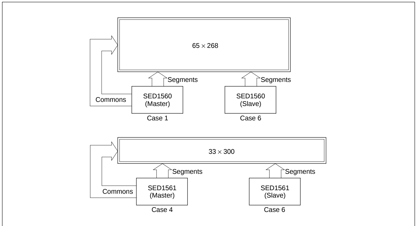
Figure 5.10 Multiple-chip combinations
