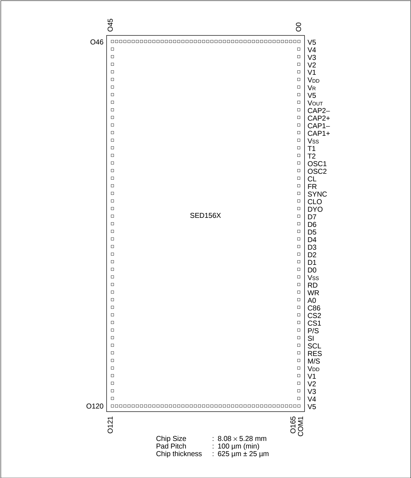
Figure 6.1 Pad layout
