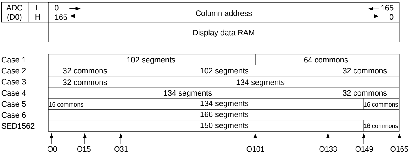
Figure 4.6 Output configuration selection
