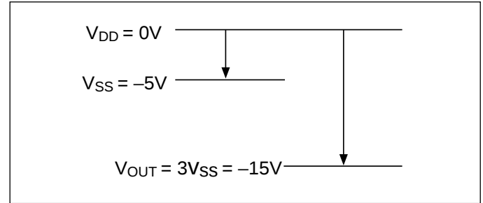
Figure 4.11 Electric potentials of triple boosting
