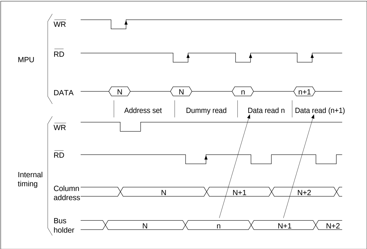
Figure 4.3 Read timing
