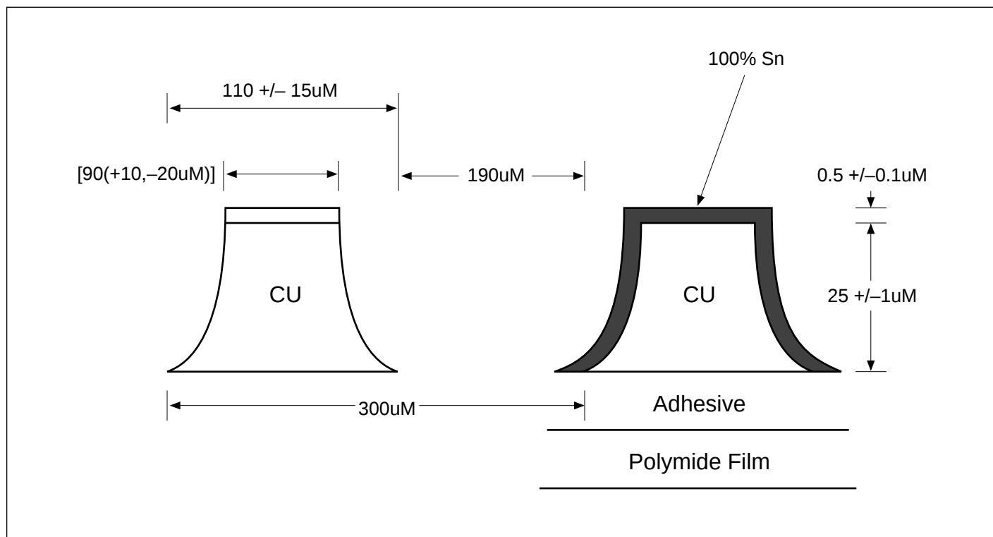
Figure 6.8 SED1560TQA OL Dimensions
