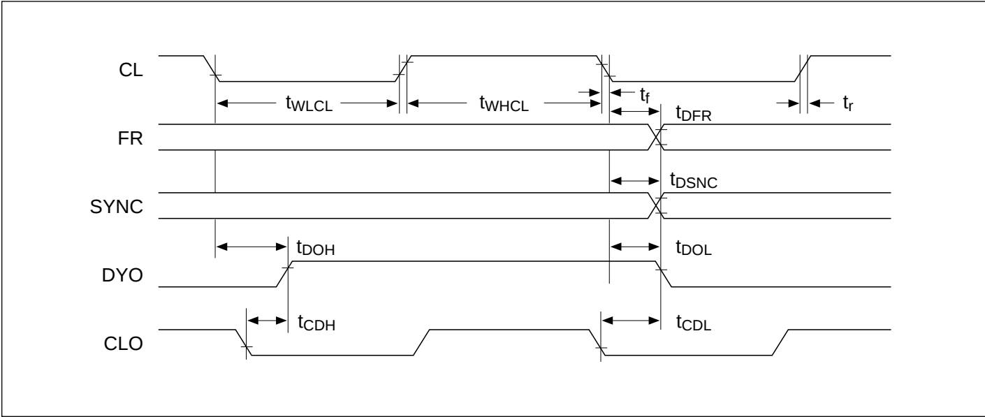
Figure 3.5 Display control timing
