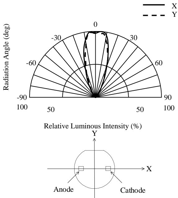
Figure 6. Directivity
