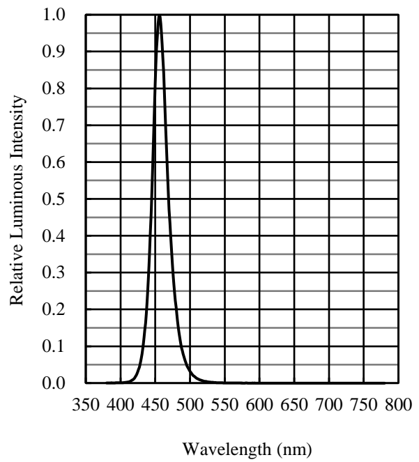
Figure 5. Spectrum
