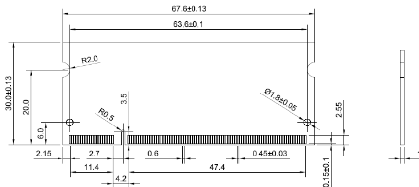
Figure: mechanical dimensions 1
