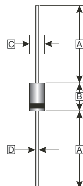
DO-41
