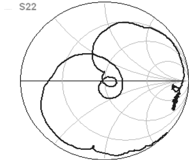
S11 and S22 Plots
