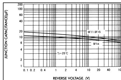
FIG.6-TYPICAL JUNCTION CAPACITANCE
