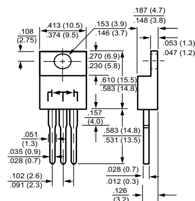
TO-220
