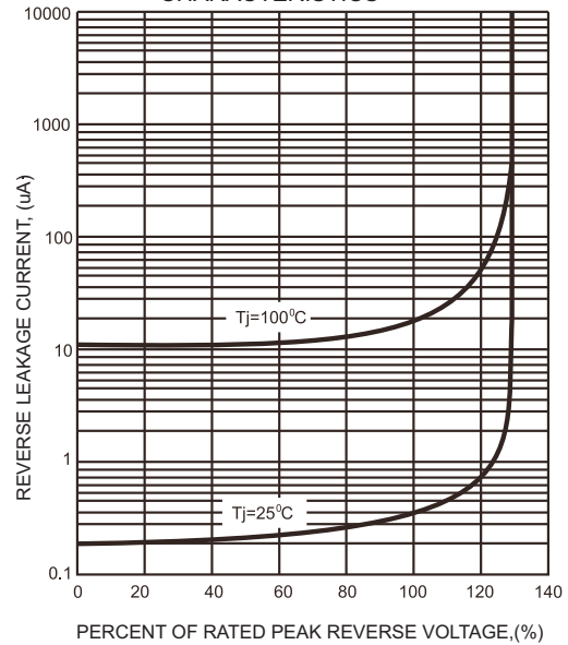
FIG.4-TYPICAL REVERSE CHARACTERISTICS
