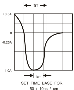
TIME CHARACTERISTIC
