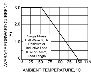
Typical Forward Current Derating Curve
